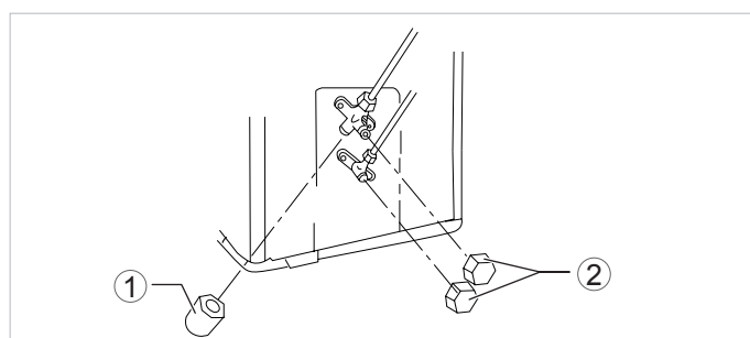
Fig. 12.7 Protective covers.
