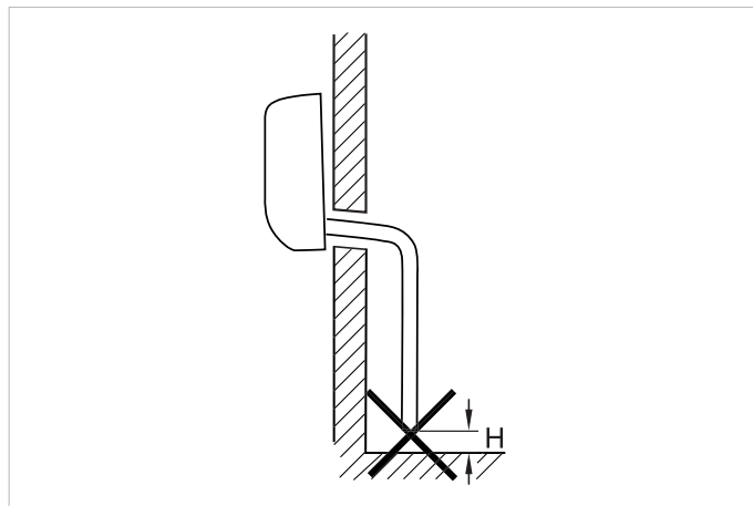
Fig. 9.4 Minimum distance from the floor.
