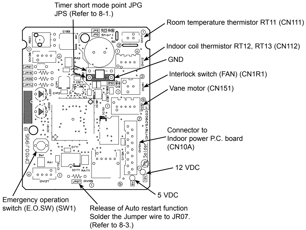
Room temperature thermistor (RT11) Indoor coil thermistor (RT12, RT13)
