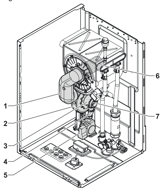
Fig.3 Gas/aire
