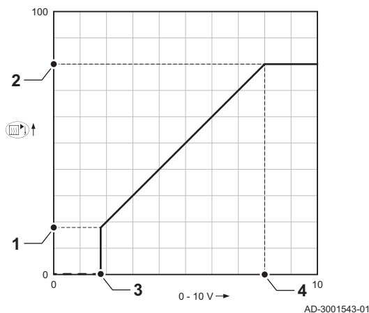
Fig.90 Control de 0-10 V
