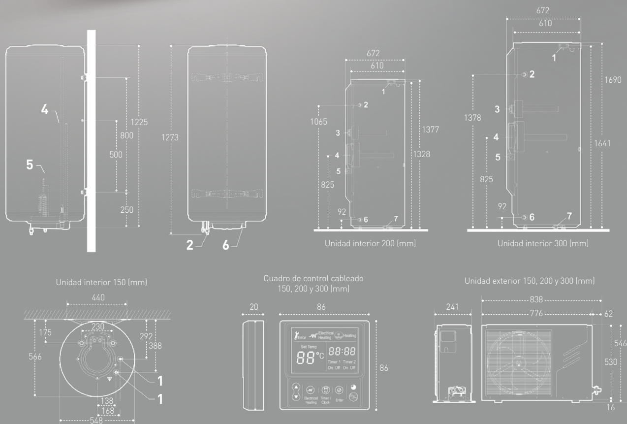
BC ACS SPLIT
